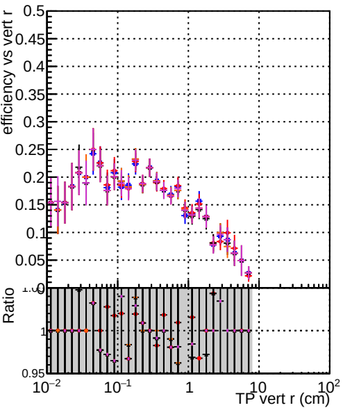
Efficiency vs TP vert r (cm) Legend: DOM original step2 ttbar-phase1-newgeom DOM pixelCPEtemplate step2 ttbar-phase1-newgeom DOM pixelCPEtemplateCutChiSquareNew step2 ttbar-phase1-newgeom DOM pixelCPEtemplateCutChiSquareNew2 step2 ttbar-phase1-newgeom DOM pixelCPEtemplateCutChiSquareNew3 step2 ttbar-phase1-newgeom
