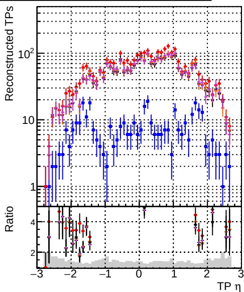
— DOM original step2 ttbar-phase1-newgeom — DOM pixelCPETemplate step2 ttbar-phase1-newgeom — DOM pixelCPETemplateCutChiSquareNew step2 ttbar-phase1-newgeom — DOM pixelCPETemplateCutChiSquareNew2 step2 ttbar-phase1-newgeom — DOM pixelCPETemplateCutChiSquareNew3 step2 ttbar-phase1-newgeom
