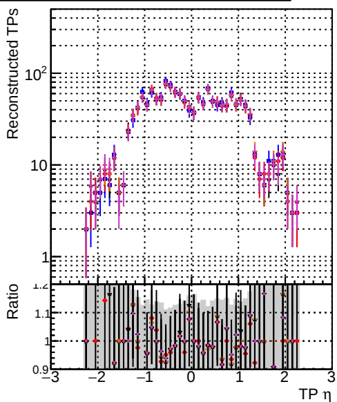
— DOM original step2 ttbar-phase1-newgeom — DOM pixelCPEtemplate step2 ttbar-phase1-newgeom — DOM pixelCPEtemplateCutChiSquareNew2 step2 ttbar-phase1-newgeom — DOM pixelCPEtemplateCutChiSquareNew3 step2 ttbar-phase1-newgeom — DOM pixelCPEtemplateCutChiSquareNew3 step2 ttbar-phase1-newgeom
