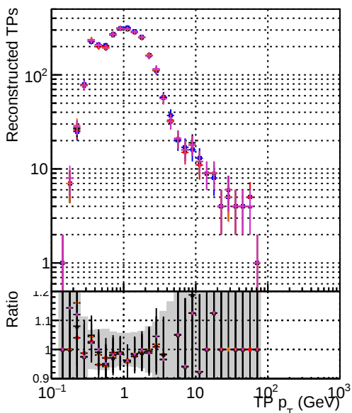
— DOM original step2 ttbar-phase1-newgeom — DOM pixelCPETemplate step2 ttbar-phase1-newgeom — DOM pixelCPETemplateCutChiSquareNew2 step2 ttbar-phase1-newgeom — DOM pixelCPETemplateCutChiSquareNew3 step2 ttbar-phase1-newgeom
