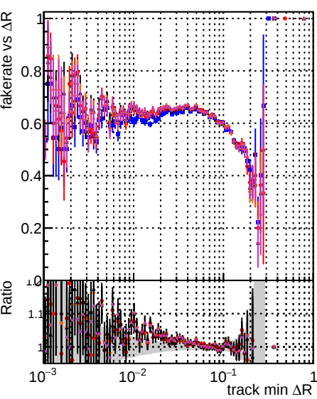
Fake rate vs \Delta R(\text{track, jet}) Legend: original (blue), step2 (red), tbar phase1 (green), newgeom (purple), and a grey shaded region for the ratio.
