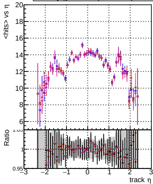
DOM original step2 ttbar-phase1-newgeom DOM pixelCPETemplate step2 ttbar-phase1-newgeom DOM pixelCPETemplateCutChiSquareNew3 step2 ttbar-phase1-newgeom DOM pixelCPETemplateCutChiSquareNew2 step2 ttbar-phase1-newgeom
