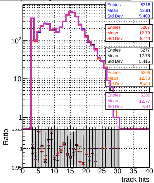
DOM original step2 ttbar-phase1-newgeom DOM pixelCPETemplate step2 ttbar-phase1-newgeom DOM pixelCPETemplateCutChiSquareNew3 step2 ttbar-phase1-newgeom DOM pixelCPETemplateCutChiSquareNew2 step2 ttbar-phase1-newgeom
