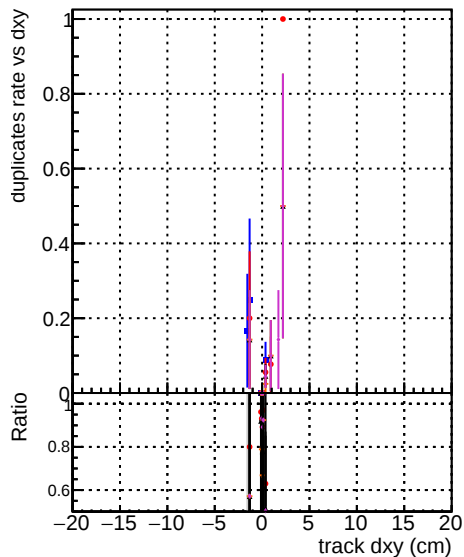
3-sqlat-new3-step2-ttbar-phase1-newgeom
