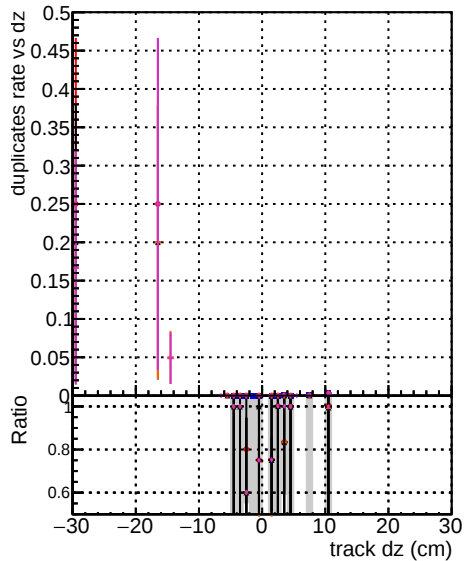
3-sqlat-new3-step2-ttbar-phase1-newgeom
