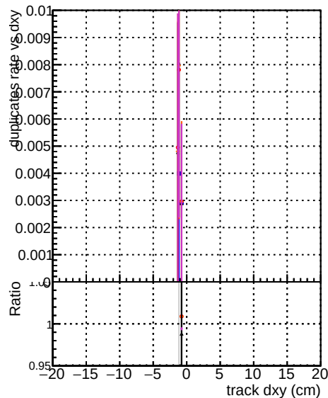
squareNews3-step2-ttbar-ph
