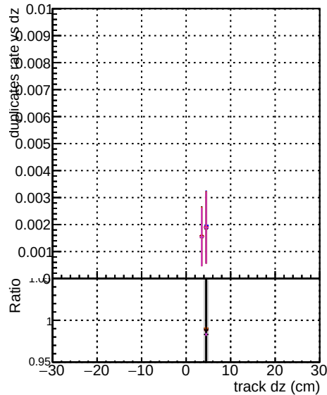
squareNews3-step2-ttbar-ph
