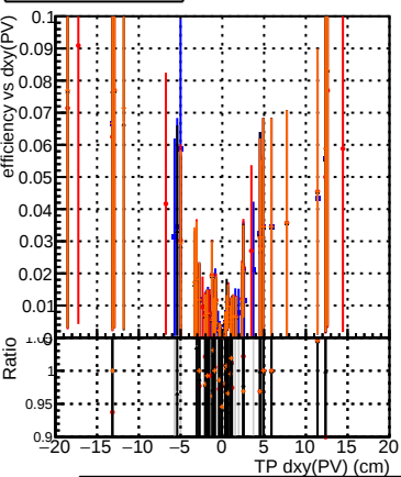
Efficiency vs Dxy(PV) Legend: DQM_original_step2_ttbar-phase1-newgeom DQM_pixelCPETemplate_step2_ttbar-phase1-newgeom DQM_pixelCPETemplateCutChiSquareNew_step2_ttbar-phase1-newgeom DQM_pixelCPETemplateCutChiSquareNew2_step2_ttbar-phase1-newgeom
