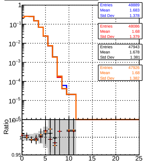
mean hits — DQM_original_step2_ttbar-phase1-newgeom — DQM_pixelCPETemplate_step2_ttbar-phase1-newgeom — DQM_pixelCPETemplateCutChiSquareNew_step2_ttbar-phase1-newgeom — DQM_pixelCPETemplateCutChiSquareNew2_step2_ttbar-phase1-newgeom
