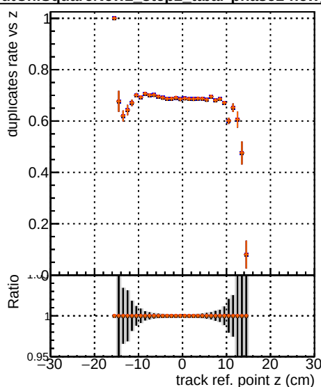
— DOM original step2 ttbar phase1 newgeom — DOM pixel CDF template step2 ttbar phase1 newgeom — DOM pixel CDF template cut chi square New2 step2 ttbar phase1 newgeom — DOM pixel CDF template cut chi square New2 step2 ttbar phase1 newgeom
