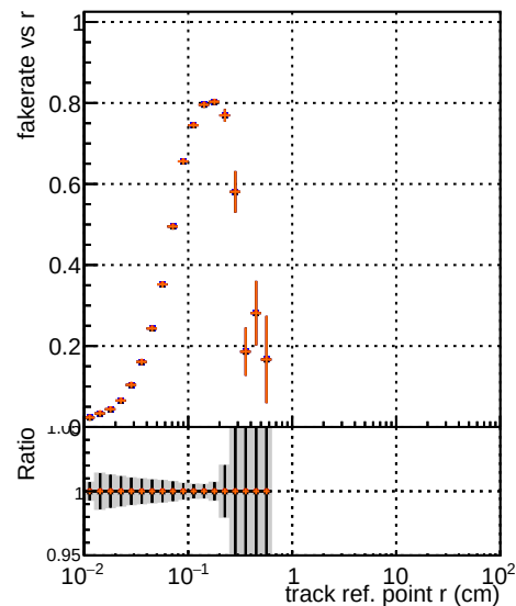
— DOM original step2 ttbar phase1 newgeom — DOM pixel CDF template step2 ttbar phase1 newgeom — DOM pixel CDF template cut chi square New2 step2 ttbar phase1 newgeom — DOM pixel CDF template cut chi square New2 step2 ttbar phase1 newgeom
