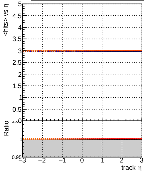
mean hits — DQM_original_step2_ttbbar-phase1-newgeom — DQM_pixelCPETemplate_step2_ttbbar-phase1-newgeom — DQM_pixelCPETemplateCutChiSquareNew_step2_ttbbar-phase1-newgeom — DQM_pixelCPETemplateCutChiSquareNew2_step2_ttbbar-phase1-newgeom
