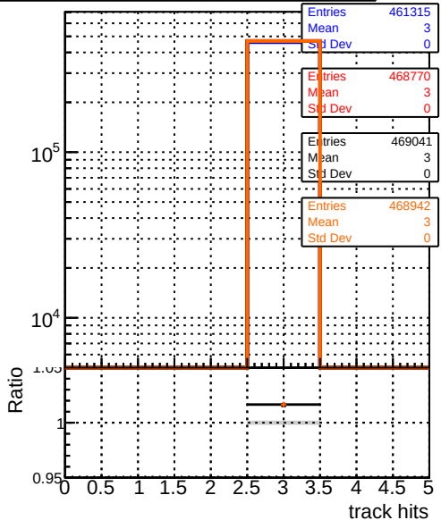
mean hits — DQM_original_step2_ttbbar-phase1-newgeom — DQM_pixelCPETemplate_step2_ttbbar-phase1-newgeom — DQM_pixelCPETemplateCutChiSquareNew_step2_ttbbar-phase1-newgeom — DQM_pixelCPETemplateCutChiSquareNew2_step2_ttbbar-phase1-newgeom
