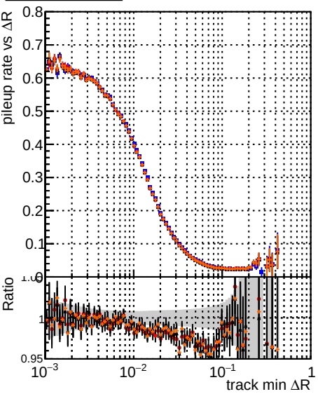
Legend: DOM original_step2_ttbbar-phase1-newgeom, DOM pixelCPE-template_step2_ttbbar-phase1-newgeom, DOM pixelCPE-template_CutChiSquareNew2_step2_ttbbar-phase1-newgeom, DOM pixelCPE-template_CutChiSquareNew2_step2_ttbbar-phase1-newgeom
