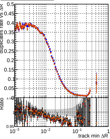
Legend: DOM original_step2_ttbbar-phase1-newgeom, DOM pixelCPE-template_step2_ttbbar-phase1-newgeom, DOM pixelCPE-template_CutChiSquareNew2_step2_ttbbar-phase1-newgeom, DOM pixelCPE-template_CutChiSquareNew2_step2_ttbbar-phase1-newgeom
