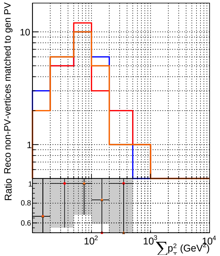
RecoAssoc2GenPVMatchedNotHighest_Pt2
