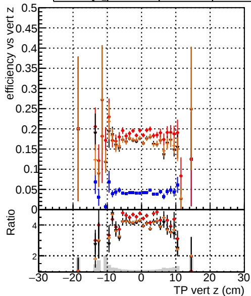
Efficiency vs vert z — DQM_original_step2_ttbare-phase1-newgeom — DQM_pixelCPETemplate_step2_ttbare-phase1-newgeom — DQM_pixelCPETemplateCutChiSquareNew_step2_ttbare-phase1-newgeom — DQM_pixelCPETemplateCutChiSquareNew2_step2_ttbare-phase1-newgeom
