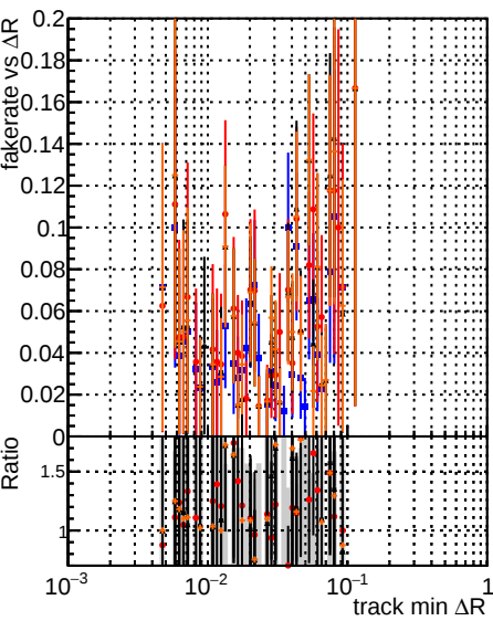
Fake rate vs \Delta R(\text{track}, \text{jet}) Legend: DOM original_step2_ttbar-phase1-newgeom, DOM pixelCPE-template_step2_ttbar-phase1-newgeom, DOM pixelCPE-template_CutChiSquareNew2_step2_ttbar-phase1-newgeom, DOM pixelCPE-template_CutChiSquareNew2_step2_ttbar-phase1-newgeom
