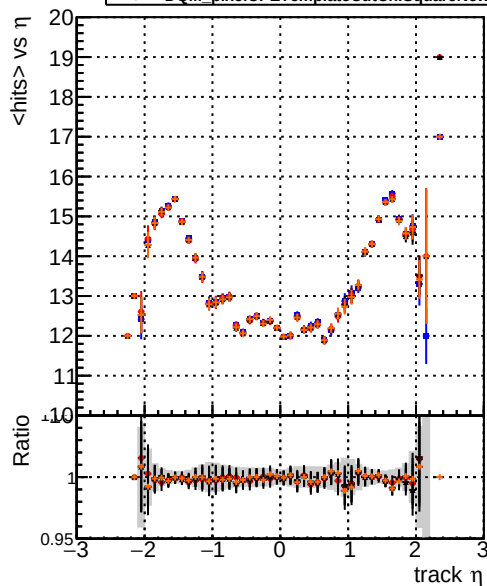
mean hits vs \eta — DQM_original_step2_ttbbar-phase1-newgeom — DQM_pixelCPETemplate_step2_ttbbar-phase1-newgeom — DQM_pixelCPETemplateCutChiSquareNew_step2_ttbbar-phase1-newgeom — DQM_pixelCPETemplateCutChiSquareNew2_step2_ttbbar-phase1-newgeom
