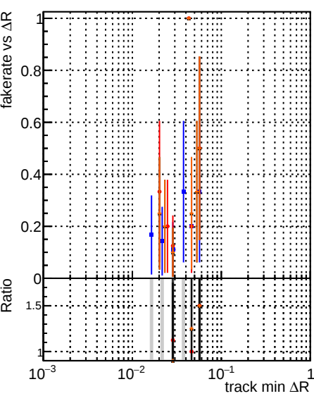
Fake rate vs \Delta R(\text{track, jet}) DOM original step2 ttbar-phase1-newgeom DOM pixelCUT step2 ttbar-phase1-newgeom DOM templateCUT step2 ttbar-phase1-newgeom DOM chiSquareNew2 step2 ttbar-phase1-newgeom
