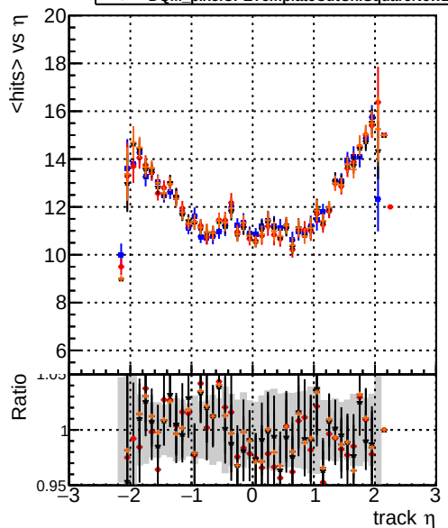
mean hits vs \eta DQM_original_step2_ttbar-phase1-newgeom DQM_pixelCPETemplate_step2_ttbar-phase1-newgeom DQM_pixelCPETemplateCutChiSquareNew_step2_ttbar-phase1-newgeom DQM_pixelCPETemplateCutChiSquareNew_step2_ttbar-phase1-newgeom
