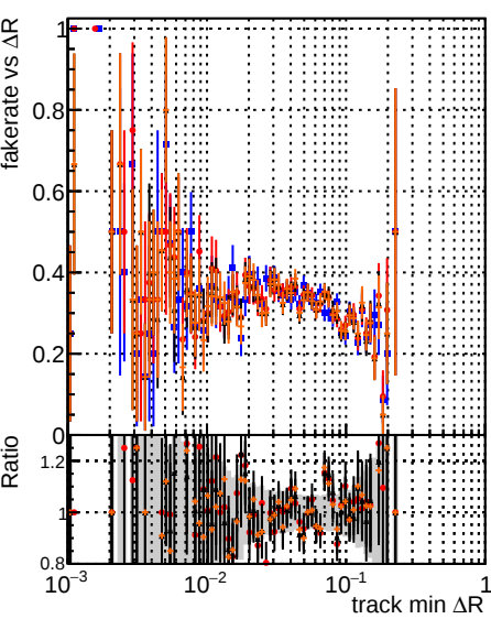
Fake rate vs \Delta R(\text{track, jet}) Legend: DOM original_step2_ttbare-phase1-newgeom DOM pixel_CDF-template_step2_ttbare-phase1-newgeom DOM pixel_CDF-template_ChiSquareNew2_step2_ttbare-phase1-newgeom DOM pixel_CDF-template_ChiSquareNew2_step2_ttbare-phase1-newgeom
