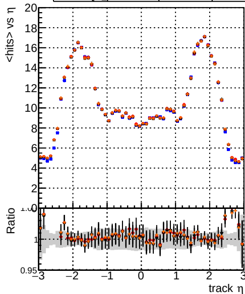
mean hits — DQM_original_step2_ttbar-phase1-newgeom — DQM_pixelCPETemplate_step2_ttbar-phase1-newgeom — DQM_pixelCPETemplateCutChiSquareNew_step2_ttbar-phase1-newgeom — DQM_pixelCPETemplateCutChiSquareNew2_step2_ttbar-phase1-newgeom
