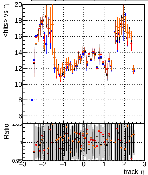
mean hits DQM_original_step2_ttbbar-phase1-newgeom DQM_pixelCPETemplate_step2_ttbbar-phase1-newgeom DQM_pixelCPETemplateCutChiSquareNew_step2_ttbbar-phase1-newgeom DQM_pixelCPETemplateCutChiSquareNew2_step2_ttbbar-phase1-newgeom
