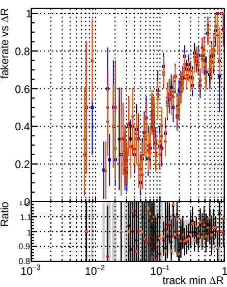
Fake rate vs \Delta R(\text{track, jet}) Legend: DOM original step2 ttbar-phase1-newgeom pixelCDE template-cut chi-square-new step2 ttbar-phase1-newgeom pixelCDE template-cut chi-square-new step2 ttbar-phase1-newgeom
