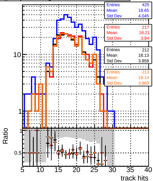
mean hits — DQM_original_step2_ttbar-phase1-newgeom — DQM_pixelCPETemplate_step2_ttbar-phase1-newgeom — DQM_pixelCPETemplateCutChiSquareNew_step2_ttbar-phase1-newgeom — DQM_pixelCPETemplateCutChiSquareNew2_step2_ttbar-phase1-newgeom
