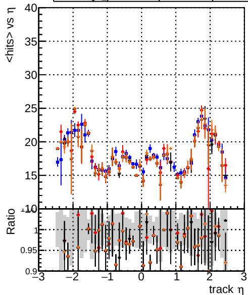
mean hits — DQM_original_step2_ttbar-phase1-newgeom — DQM_pixelCPETemplate_step2_ttbar-phase1-newgeom — DQM_pixelCPETemplateCutChiSquareNew_step2_ttbar-phase1-newgeom — DQM_pixelCPETemplateCutChiSquareNew2_step2_ttbar-phase1-newgeom
