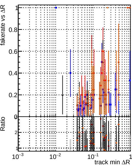
Fake rate vs ΔR(track, jet) Legend: DOM (blue), original (red), step2 (black), ttbar-phase1-newgeom (orange), pixelCP (grey), ETemplate (green), CutChiSquareNew (purple), step2 ttbar-phase1-newgeom (brown).
