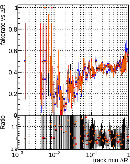
Fake rate vs \Delta R (track, jet) Legend: DOM original (blue squares) DOM pixel (red circles) DOM pixel CDF template (black triangles) DOM pixel CDF template cut (orange diamonds) DOM pixel CDF template cut chi square New2 (green crosses)
