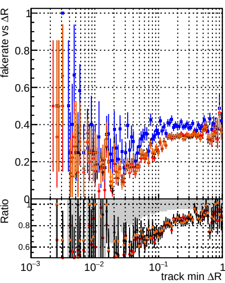
Fake rate vs \Delta R (track, jet) | Duplicates Rate vs \Delta R (track, jet) | Pileup rate vs \Delta R (track, jet) Legend for all plots: DOM original (blue squares) DOM pixelCDE template (red circles) DOM pixelCDE template cut (black triangles) DOM pixelCDE template cut chiSquareNew2 (orange diamonds)
