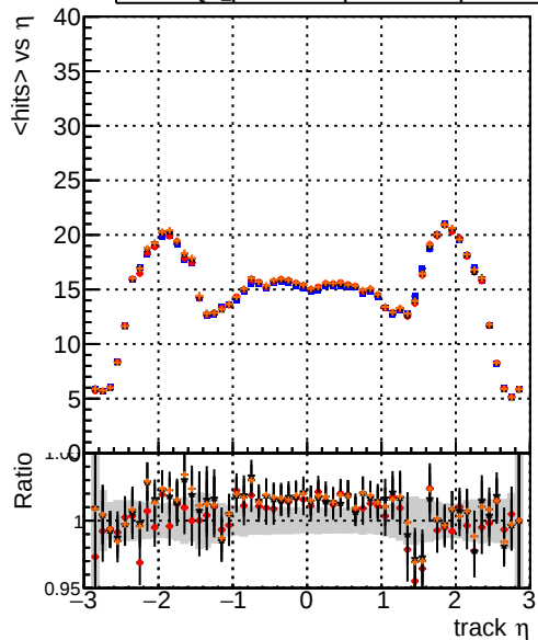
Legend: — DQM_original_step2_ttbar-phase1-newgeom — DQM_pixelCPETemplate_step2_ttbar-phase1-newgeom — DQM_pixelCPETemplateCutChiSquareNew_step2_ttbar-phase1-newgeom — DQM_pixelCPETemplateCutChiSquareNew2_step2_ttbar-phase1-newgeom mean hits
