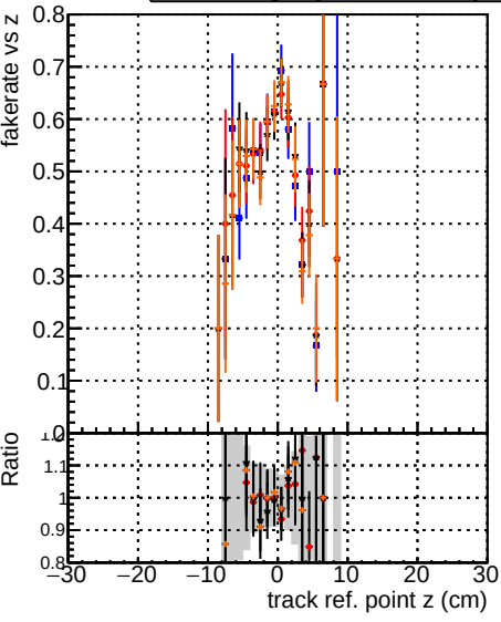
Fake rate vs z
