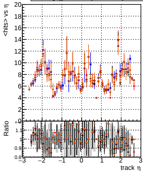
mean hits vs \eta Legend: Blue line: DQM_original_step2_ttbbar-phase1-newgeom Red line: DQM_pixelCPETemplate_step2_ttbbar-phase1-newgeom Black line: DQM_pixelCPETemplateCutChiSquareNew_step2_ttbbar-phase1-newgeom Orange line: DQM_pixelCPETemplateCutChiSquareNew2_step2_ttbbar-phase1-newgeom
