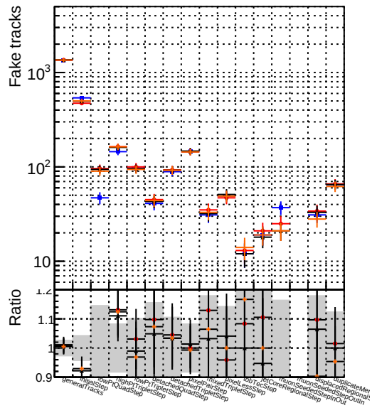
Number of tracks vs collection DQM_original_step2_ttbar-phase1-newgeom DQM_pixelCPETemplate_step2_ttbar-phase1-newgeom DQM_pixelCPETemplateCutChiSquareNew_step2_ttbar-phase1-newgeom DQM_pixelCPETemplateCutChiSquareNew2_step2_ttbar-phase1-newgeom
