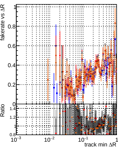
Fake rate vs \Delta R(\text{track, jet}) DOM original_step2_ttbare-phase1-newgeom DOM pixel_CDF_template_step2_ttbare-phase1-newgeom DOM pixel_CDF_template_chiSquareNew2_step2_ttbare-phase1-newgeom DOM pixel_CDF_templateCutChiSquareNew2_step2_ttbare-phase1-newgeom
