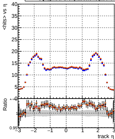
mean hit DQM_original_step2_ttbar-phase1-newgeom DQM_pixelCPETemplate_step2_ttbar-phase1-newgeom DQM_pixelCPETemplateCutChiSquareNew_step2_ttbar-phase1-newgeom DQM_pixelCPETemplateCutChiSquareNew2_step2_ttbar-phase1-newgeom
