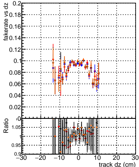
— DGM original_step2_tbar_phase1_newgeom — DGM pixel_CPE_template_step2_tbar_phase1_newgeom — DGM pixel_CPE_template_CurChiSquareNew2_step2_tbar_phase1_newgeom — Ratio
