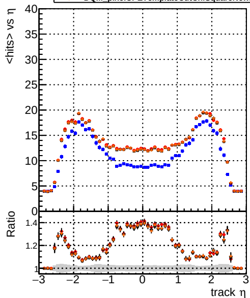
mean hits vs \eta — DQM_original_step2_ttbar-phase1-newgeom — DQM_pixelCPETemplate_step2_ttbar-phase1-newgeom — DQM_pixelCPETemplateCutChiSquareNew_step2_ttbar-phase1-newgeom — DQM_pixelCPETemplateCutChiSquareNew2_step2_ttbar-phase1-newgeom
