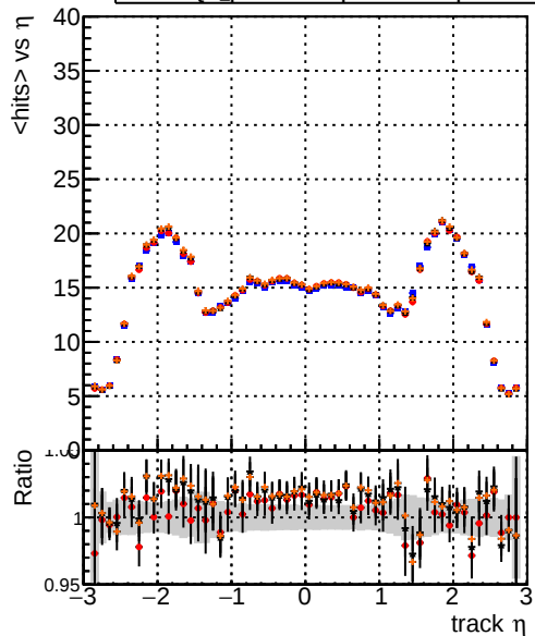
mean hit DQM_original_step2_ttbar-phase1-newgeom DQM_pixelCPETemplate_step2_ttbar-phase1-newgeom DQM_pixelCPETemplateCutChiSquareNew_step2_ttbar-phase1-newgeom DQM_pixelCPETemplateCutChiSquareNew2_step2_ttbar-phase1-newgeom
