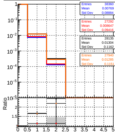
mean hit DQM_original_step2_ttbar-phase1-newgeom DQM_pixelCPETemplate_step2_ttbar-phase1-newgeom DQM_pixelCPETemplateCutChiSquareNew_step2_ttbar-phase1-newgeom DQM_pixelCPETemplateCutChiSquareNew2_step2_ttbar-phase1-newgeom
