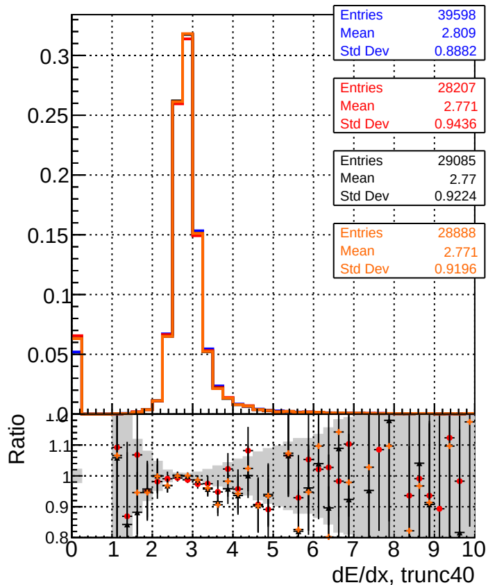
— DQM_original_step2_ttbar-phase1-newgeom — DQM_pixelCPETemplate_step2_ttbar-phase1-newgeom — DQM_pixelCPETemplateCutChiSquareNew_step2_ttbar-phase1-newgeom — DQM_pixelCPETemplateCutChiSquareNew2_step2_ttbar-phase1-newgeom
