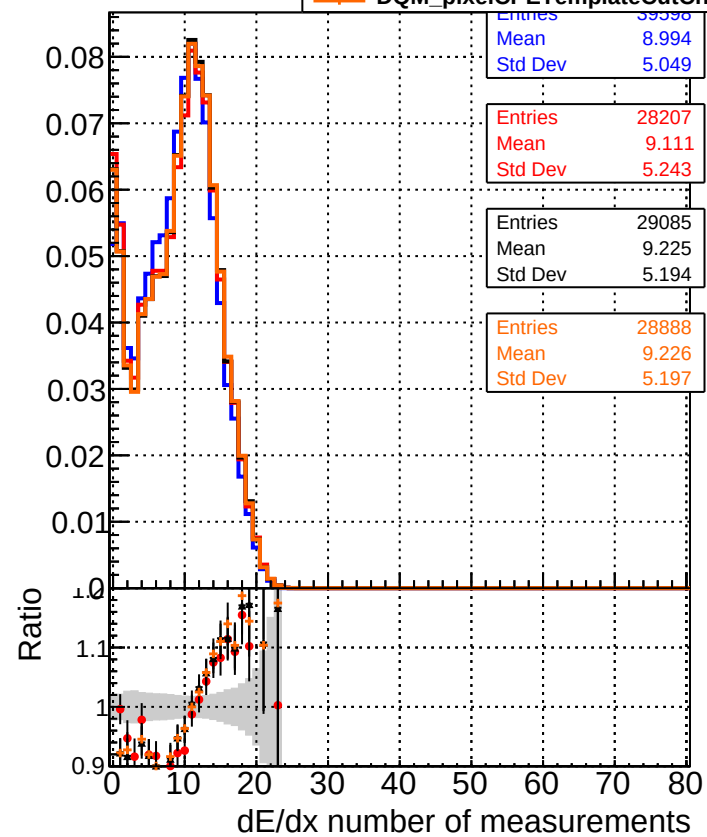
— DQM_original_step2_ttbar-phase1-newgeom — DQM_pixelCPETemplate_step2_ttbar-phase1-newgeom — DQM_pixelCPETemplateCutChiSquareNew_step2_ttbar-phase1-newgeom — DQM_pixelCPETemplateCutChiSquareNew2_step2_ttbar-phase1-newgeom
