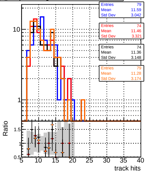
mean hit — DQM_original_step2_ttbar-phase1-newgeom — DQM_pixelCPETemplate_step2_ttbar-phase1-newgeom — DQM_pixelCPETemplateCutChiSquareNew_step2_ttbar-phase1-newgeom — DQM_pixelCPETemplateCutChiSquareNew_step2_ttbar-phase1-newgeom
