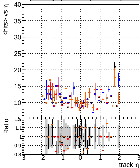
mean hit — DQM_original_step2_ttbar-phase1-newgeom — DQM_pixelCPETemplate_step2_ttbar-phase1-newgeom — DQM_pixelCPETemplateCutChiSquareNew_step2_ttbar-phase1-newgeom — DQM_pixelCPETemplateCutChiSquareNew_step2_ttbar-phase1-newgeom
