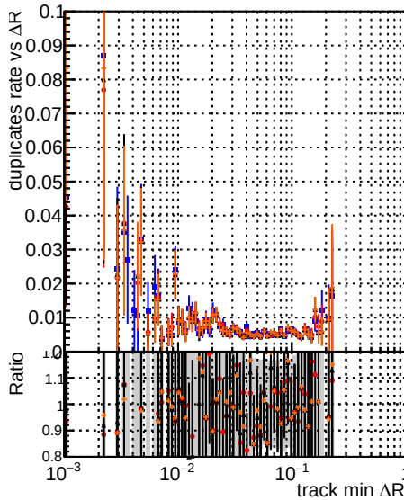
— original_step2_ttbbar-phase1-newgeom — pixelCDE-template_step2_ttbbar-phase1-newgeom — pixelCDE-template_CutChiSquareNew2_step2_ttbbar-phase1-newgeom — pixelCDE-template_CutChiSquareNew2_step2_ttbbar-phase1-newgeom
