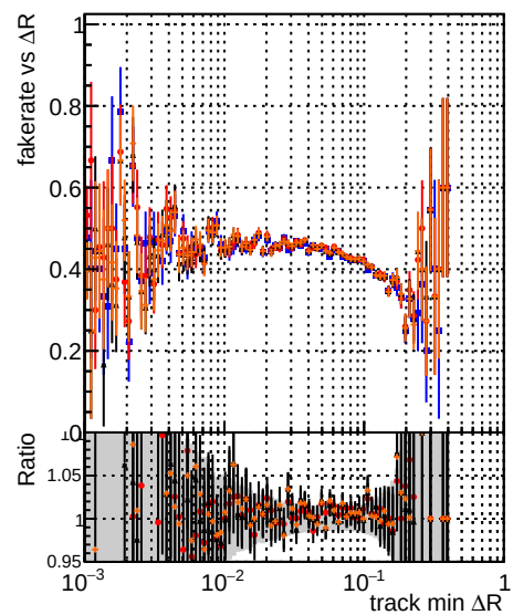
— original_step2_ttbbar-phase1-newgeom — pixelCDE-template_step2_ttbbar-phase1-newgeom — pixelCDE-template_CutChiSquareNew2_step2_ttbbar-phase1-newgeom — pixelCDE-template_CutChiSquareNew2_step2_ttbbar-phase1-newgeom
