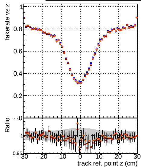
DOM original step2 ttbar phase1-newgeom DOM pixelCPE template step2 ttbar phase1-newgeom DOM pixelCPE template ChiSquareNew2 step2 ttbar phase1-newgeom
