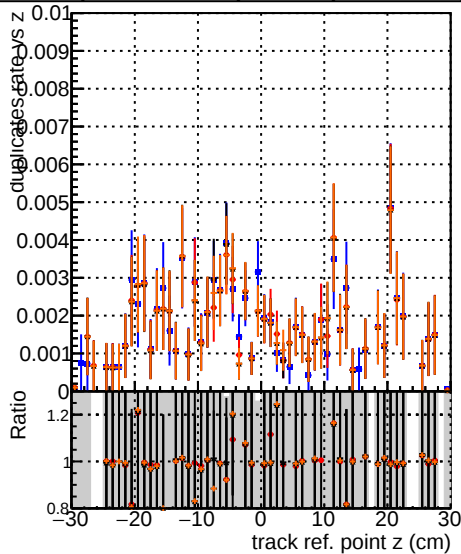
DOM original step2 ttbar phase1-newgeom DOM pixelCPE template step2 ttbar phase1-newgeom DOM pixelCPE template ChiSquareNew2 step2 ttbar phase1-newgeom
