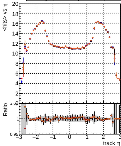
mean hits vs \eta — DQM_original_step2_ttbare-phase1-newgeom — DQM_pixelCPETemplate_step2_ttbare-phase1-newgeom — DQM_pixelCPETemplateCutChiSquareNew_step2_ttbare-phase1-newgeom — DQM_pixelCPETemplateCutChiSquareNew2_step2_ttbare-phase1-newgeom
