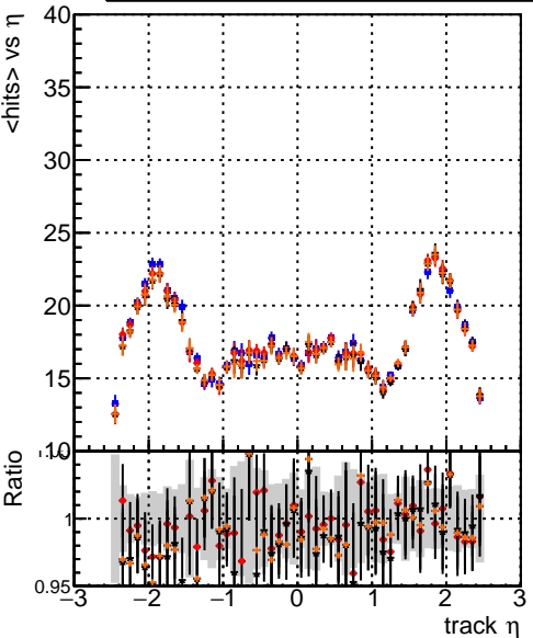
mean hit \eta Legend: Blue line: DQM_original_step2_ttbar-phase1-newgeom Red line: DQM_pixelCPETemplate_step2_ttbar-phase1-newgeom Black line: DQM_pixelCPETemplateCutChiSquareNew_step2_ttbar-phase1-newgeom Orange line: DQM_pixelCPETemplateCutChiSquareNew_step2_ttbar-phase1-newgeom
