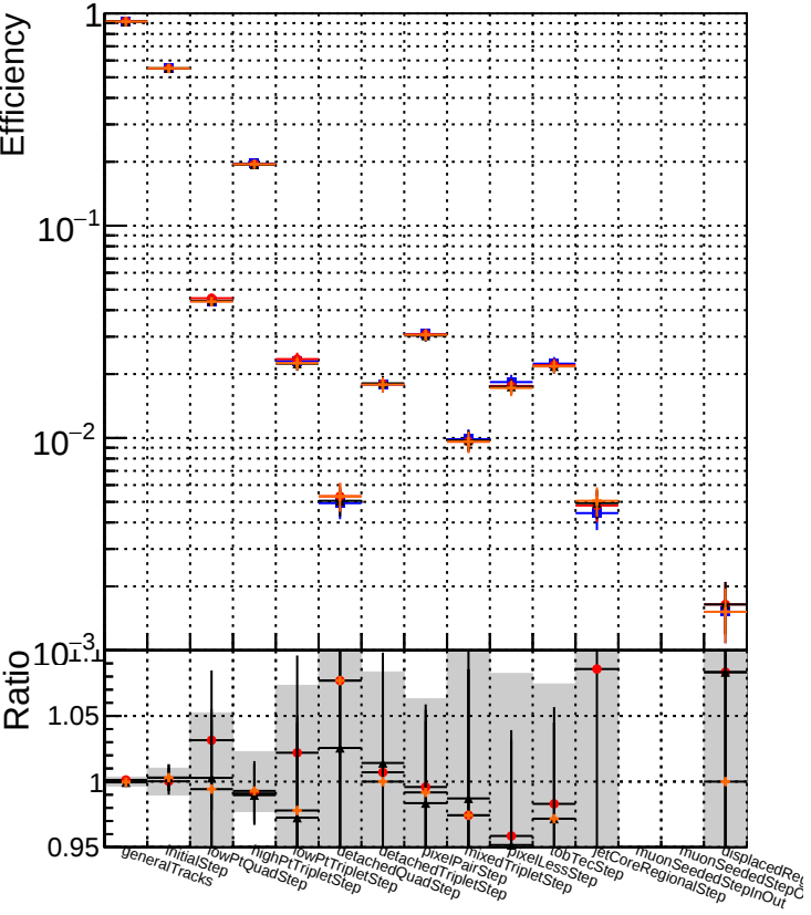
DQM_original_step2_ttbar-phase1-newgeom DQM_pixelCPETemplate_step2_ttbar-phase1-newgeom DQM_pixelCPETemplateCutChiSquareNew_step2_ttbar-phase1-newgeom DQM_pixelCPETemplateCutChiSquareNew2_step2_ttbar-phase1-newgeom
