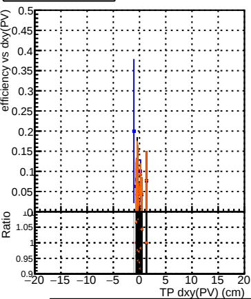
Efficiency vs Dxy(PV) DQM_original_step2_ttbar-phase1-newgeom DQM_pixelCPETemplate_step2_ttbar-phase1-newgeom DQM_pixelCPETemplateCutChiSquareNew_step2_ttbar-phase1-newgeom DQM_pixelCPETemplateCutChiSquareNew2_step2_ttbar-phase1-newgeom
