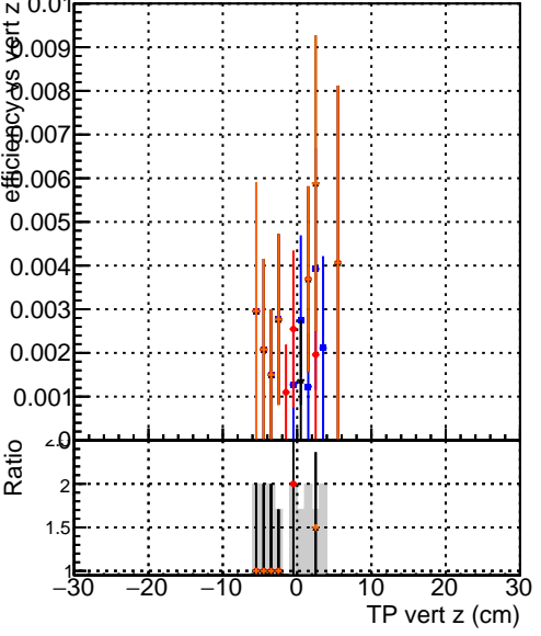
Efficiency vs TP vert z DQM_original_step2_ttbar-phase1-newgeom DQM_pixelCPETemplate_step2_ttbar-phase1-newgeom DQM_pixelCPETemplateCutChiSquareNew_step2_ttbar-phase1-newgeom DQM_pixelCPETemplateCutChiSquareNew2_step2_ttbar-phase1-newgeom
