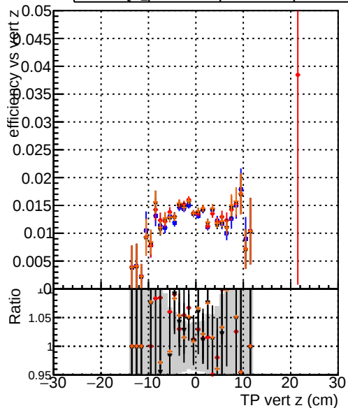
Efficiency vs. TP vert z — DQM_original_step2_ttbare-phase1-newgeom — DQM_pixelCPETemplate_step2_ttbare-phase1-newgeom — DQM_pixelCPETemplateCutChiSquareNew_step2_ttbare-phase1-newgeom — DQM_pixelCPETemplateCutChiSquareNew2_step2_ttbare-phase1-newgeom
