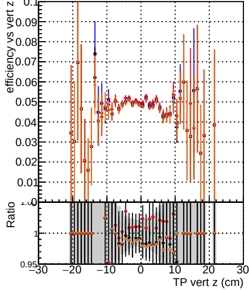
Efficiency vs. TP vert z — DQM_original_step2_ttbar-phase1-newgeom — DQM_pixelCPETemplate_step2_ttbar-phase1-newgeom — DQM_pixelCPETemplateCutChiSquareNew_step2_ttbar-phase1-newgeom — DQM_pixelCPETemplateCutChiSquareNew2_step2_ttbar-phase1-newgeom
