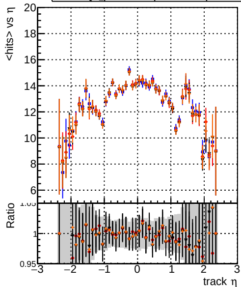
mean hits DQM_originalStep2_ttbar-phase1-newgeom DQM_pixelCPETemplate_step2_ttbar-phase1-newgeom DQM_pixelCPETemplateCutChiSquareNew_step2_ttbar-phase1-newgeom DQM_pixelCPETemplateCutChiSquareNew_step2_ttbar-phase1-newgeom
