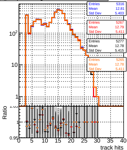
mean hits DQM_originalStep2_ttbar-phase1-newgeom DQM_pixelCPETemplate_step2_ttbar-phase1-newgeom DQM_pixelCPETemplateCutChiSquareNew_step2_ttbar-phase1-newgeom DQM_pixelCPETemplateCutChiSquareNew_step2_ttbar-phase1-newgeom
