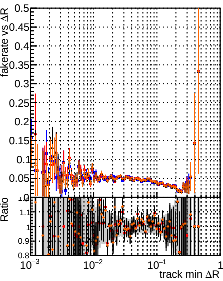
Fake rate vs \Delta R(\text{track}, \text{jet}) DOM original_step2_ttbbar-phase1-newgeom DOM pixelCBETemplate_step2_ttbbar-phase1-newgeom DOM pixelCBETemplateCutChiSquareNew2_step2_ttbbar-phase1-newgeom DOM pixelCBETemplateCutChiSquareNew2_step2_ttbbar-phase1-newgeom
