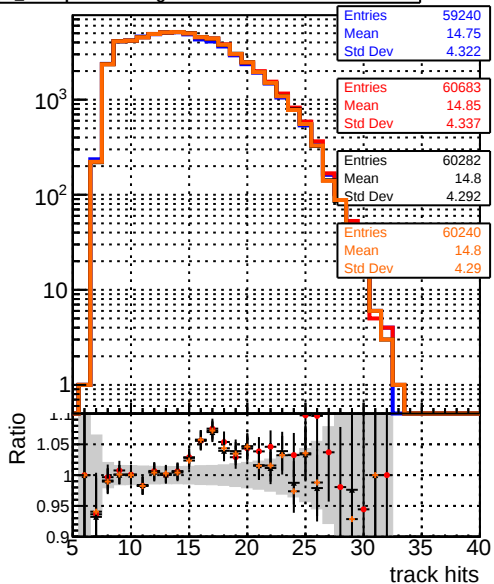
— DQM_original_step2_ttbare-phase1-newgeom — DQM_pixelCPETemplate_step2_ttbare-phase1-newgeom — DQM_pixelCPETemplateCutChiSquareNew_step2_ttbare-phase1-newgeom — DQM_pixelCPETemplateCutChiSquareNew2_step2_ttbare-phase1-newgeom
